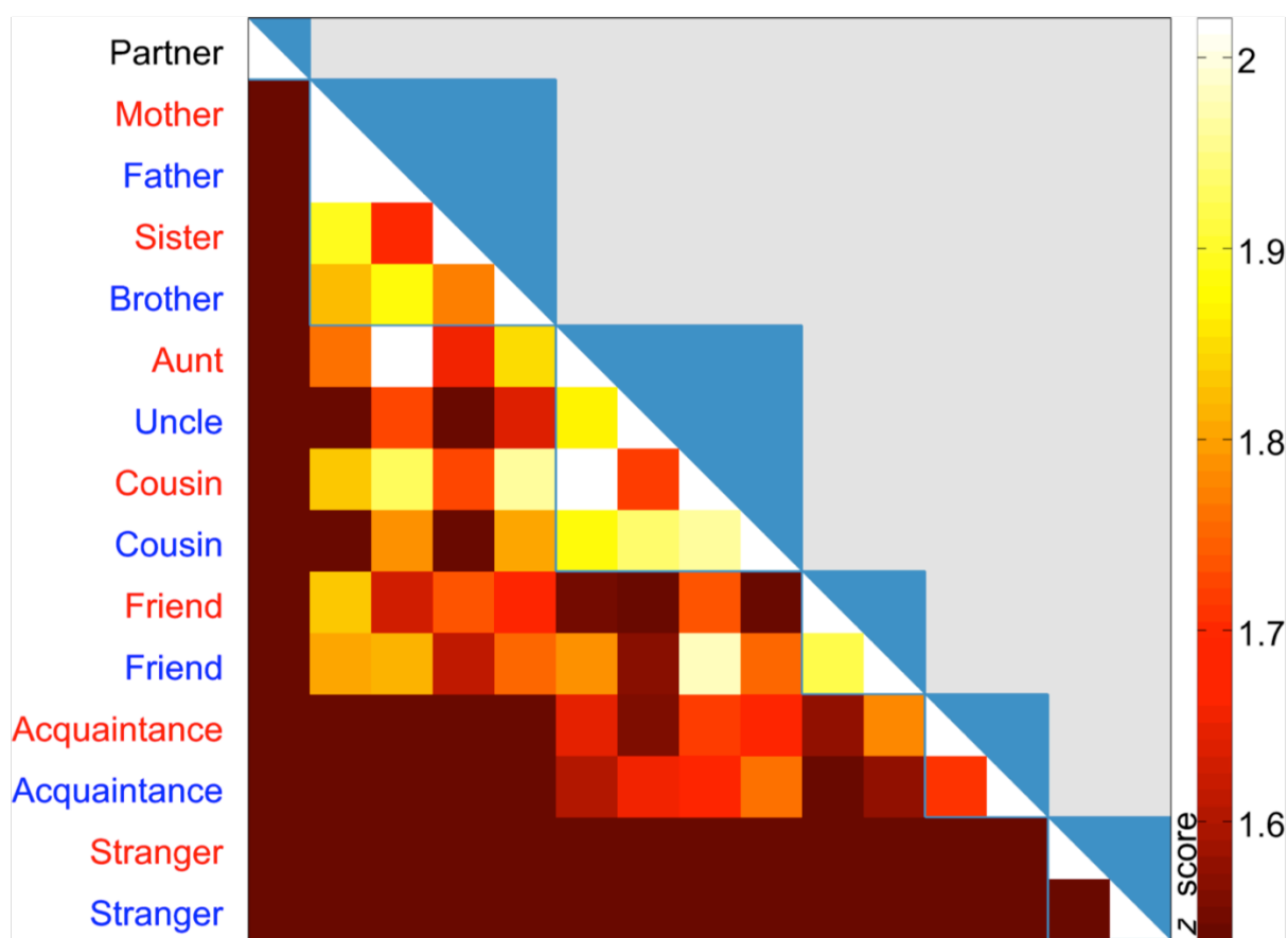
Figure S6: Touching-allowance-based similarity between members in the social network. The adjacency matrix is symmetric, and the same order of labels holds for the horizontal axis. Lower triangular matrix shows the z-transformed Spearman correlation between the average spatial maps. Upper triangular matrix demonstrates the a priori social network layers (from left to right: family, family of origin, extended family, friends, acquaintances, and strangers). Within each ideal network block, the block (light blue) is assumed to be fully correlated and have zero correlation elsewhere (light grey areas). For visualization purposes, the figure only shows values exceeding the median across all map pairs. Blue and red labels signify males and females respectively.
